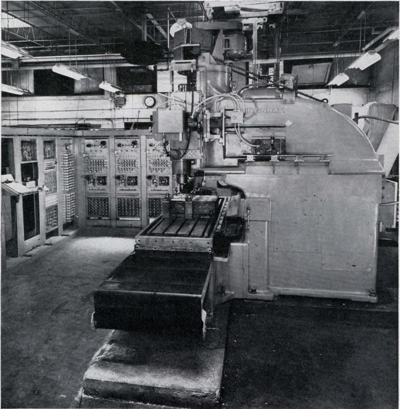
MACHINE AND CONTROL are shown here in entirety. For details of the control panels ( left ) see pages 104 and 105. The machine has universal motion: the "head," holding the cutting tool, moves vertically; the "cross
