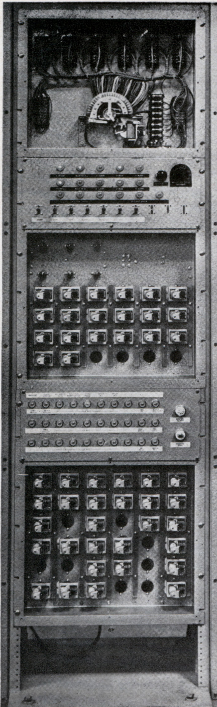
CONTROL-SYSTEM panel at left distributes commands to banks of relays in three panels at right, one for
